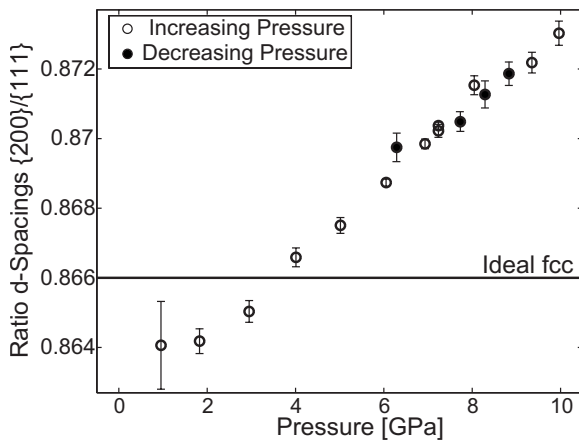
FIG. 4. Plot of the ratio of the d spacings of the {200} peak to the {111} peak. This silver nanoparticle sample was 7.2 nm in diameter and was loaded in 1:1 pentane:isopentane under an argon atmosphere. Solid line corresponds to the ratio of an ideal fcc structure (0.866). This plot clearly demonstrates noncubic distortion with increasing pressure.
