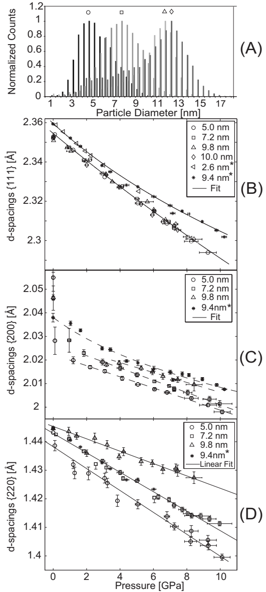
FIG. 5. d spacings as a function of measured pressure. (A) Shows a histogram of nanoparticle sizes of the Ag samples not exposed to oxygen. (B), (C), and (D) are plots of the {111}, {200}, and {220} d spacings with pressure, respectively. Lines are drawn on (B), (C), and (D) as guides for the eyes. Samples labeled with * were exposed to oxygen during sample loading.
