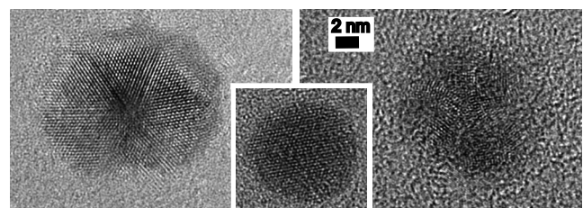
FIG. 2. Representative high-resolution TEM images of silver nanoparticles used in the x-ray diffraction experiments. The samples used in this study primarily possessed multiply twinned domains (left and right images); however, single-crystal particles were occasionally observed (center image).
