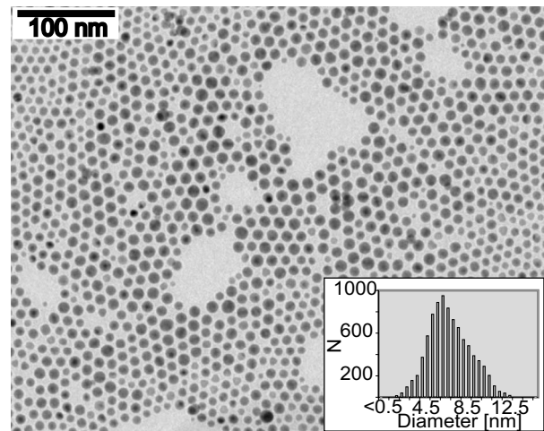
FIG. 1. TEM of the 7.2 nm silver sample used in the x-ray diffraction. Histogram of nanoparticle size distribution is shown in the inset.
