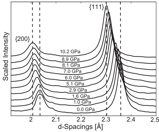
FIG. 3. Stacked plot of the x-ray diffraction patterns of 9.4 nm silver nanoparticles compressed in a DAC from 0 to 10 GPa. The relative shifts of the {111} and the {200} peaks are not the same with pressure. Dashed lines are drawn as guides for the eyes.
